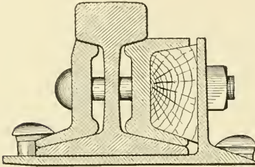
Fig. 227. Weber Joint
